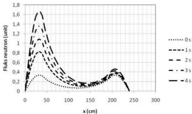
Gambar 2 Fluks penampang
